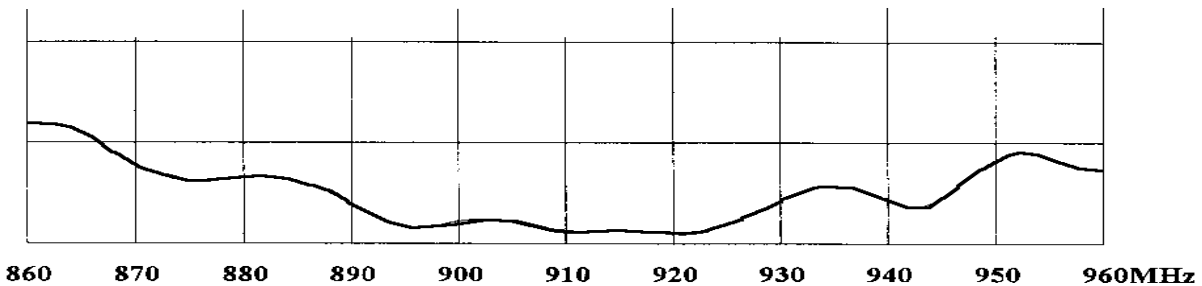
VSWR v Freq (MHz)
