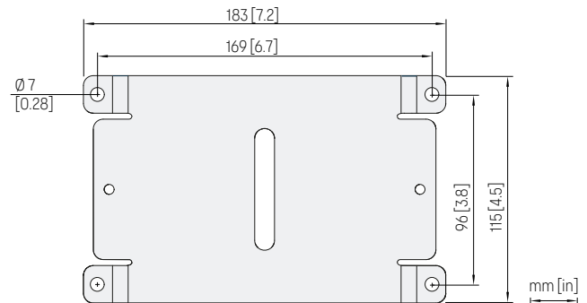
Indigo500 retrofit mounting plate dimensions
